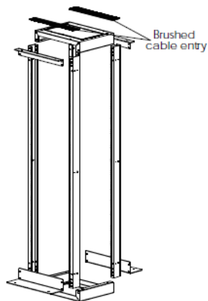
EXPLODED VIEW
